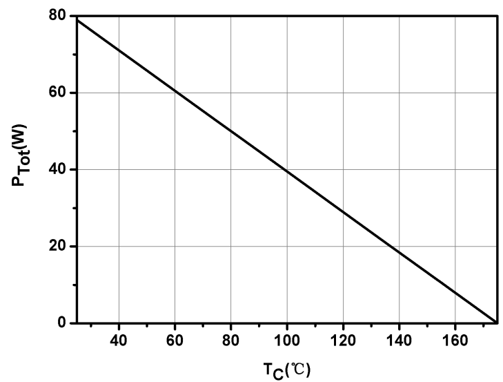
Fig.6-Power Derating
